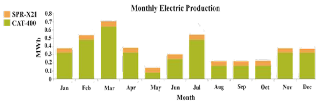
Fig. 8: The monthly electrical production of the system
